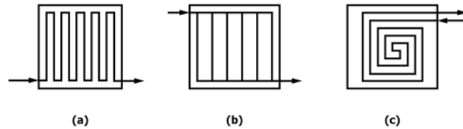
FIG. X1.1 Some Layouts of the Liquid Paths in Heating or Cooling Plates
