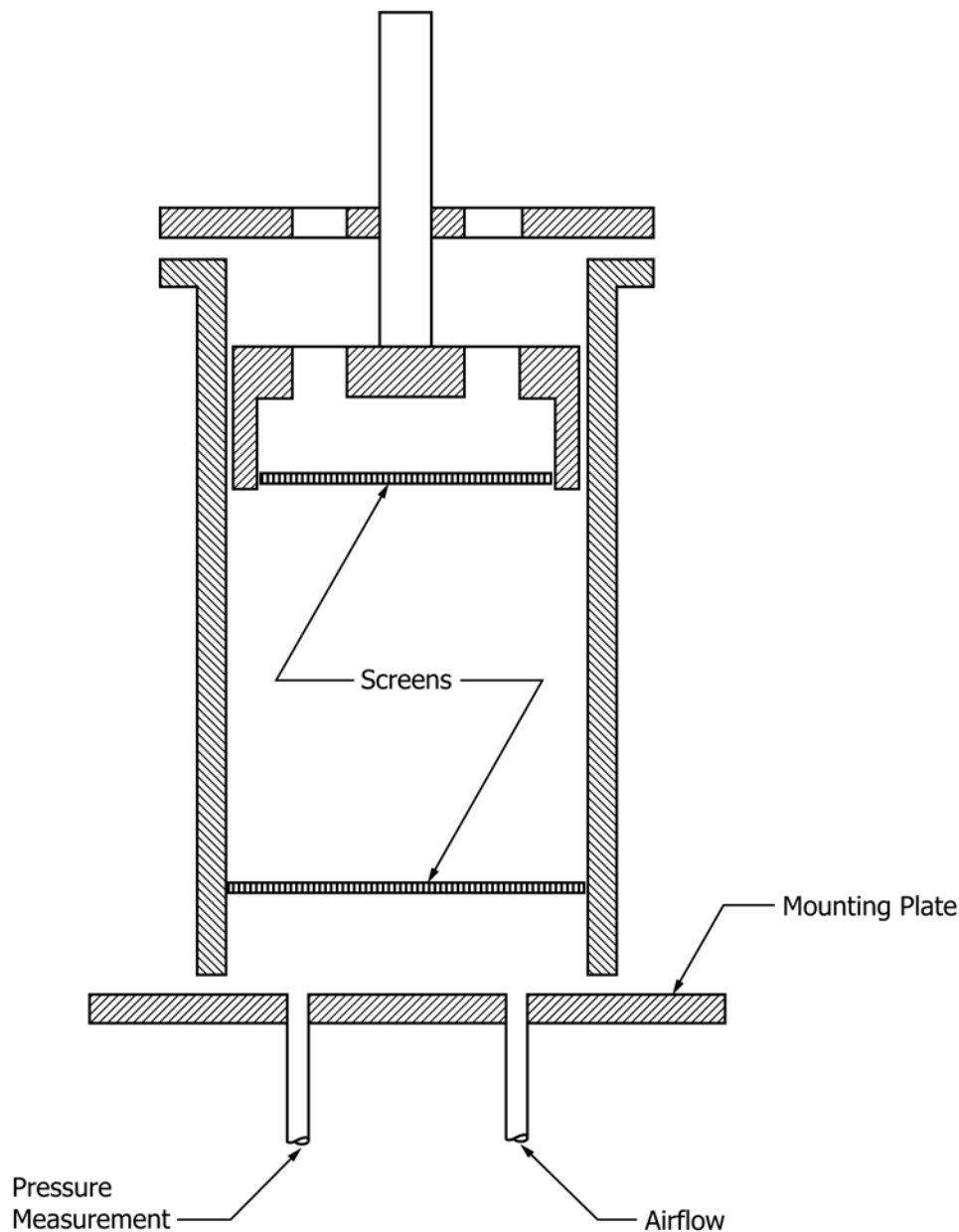
FIG. 2 Specimen Holder
