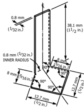
C. MOLDED CORNER (INSIDE)
