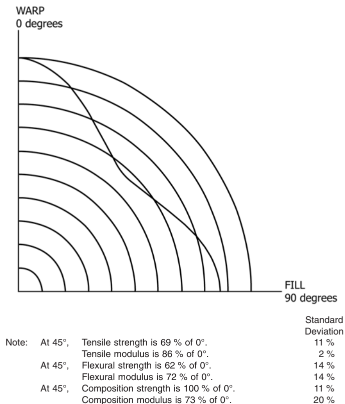
FIG. X1.1 Directional Properties of RTP Alternating Mat/Woven Roving
