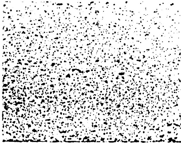
FIG. 1 Reboiling of Porcelain Enamel on Steel
