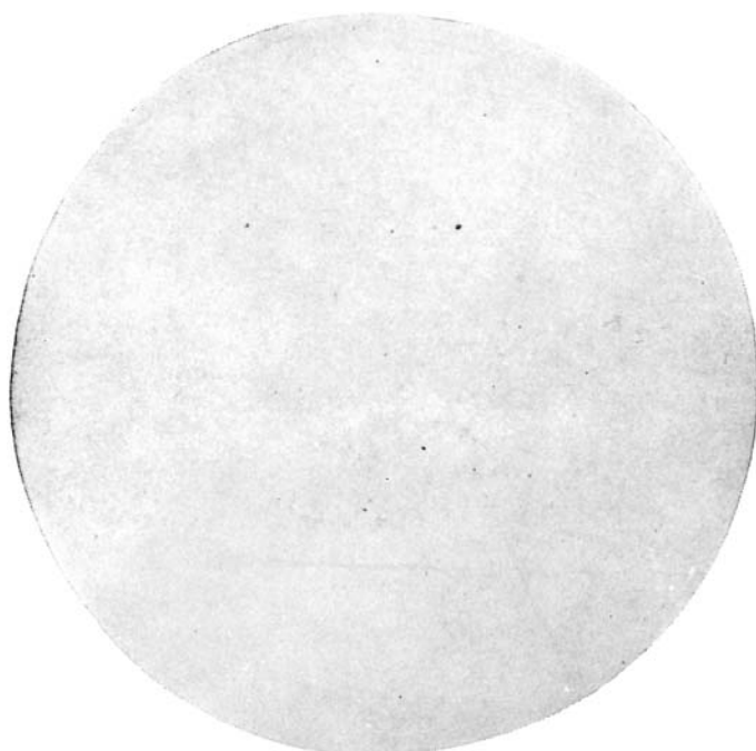
Stain Index = 20
