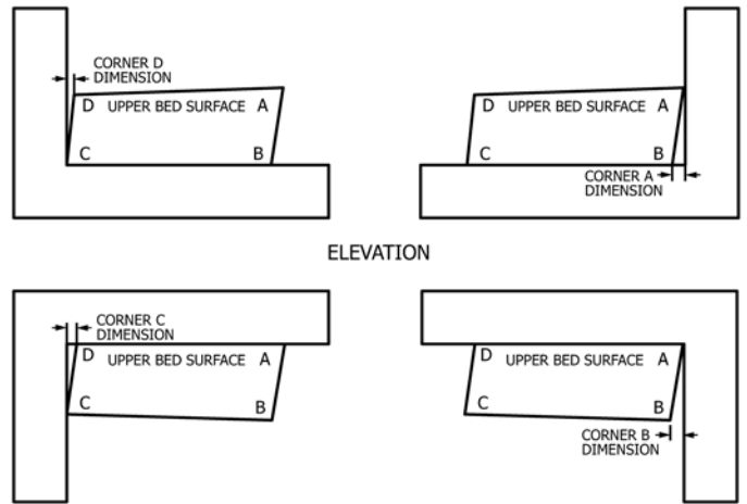
FIG. 5 Out-of-Square Measurements
