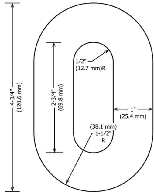
FIG. 4 Test Specimen
