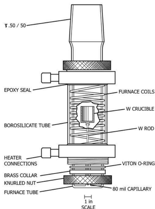
FIG. 7 Induction Furnace
