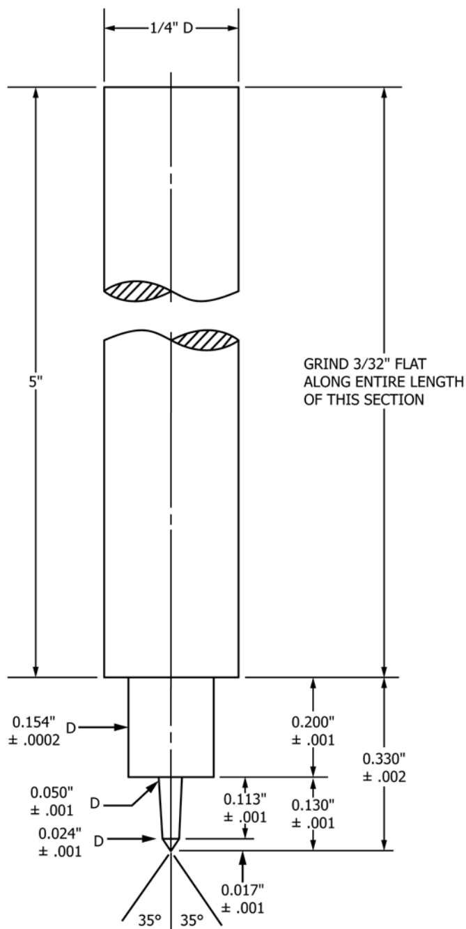
FIG. 6 Venting Tool
