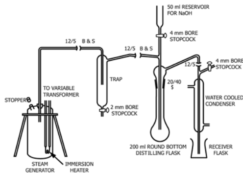
FIG. 1 Distillation Apparatus
