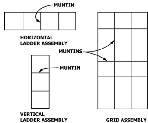
FIG. 1 Gasket Systems
