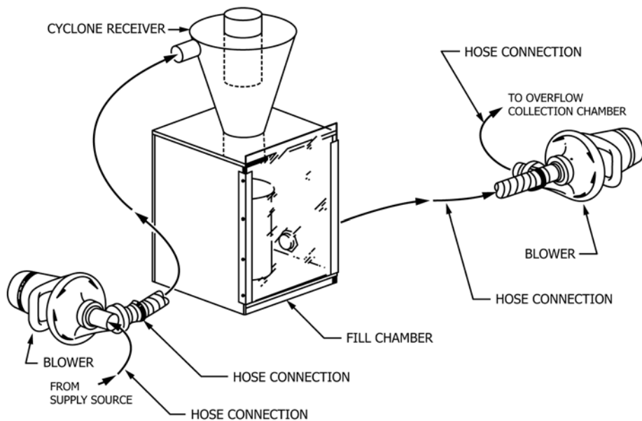
FIG. 1 Partial Insulation Preparation Apparatus
