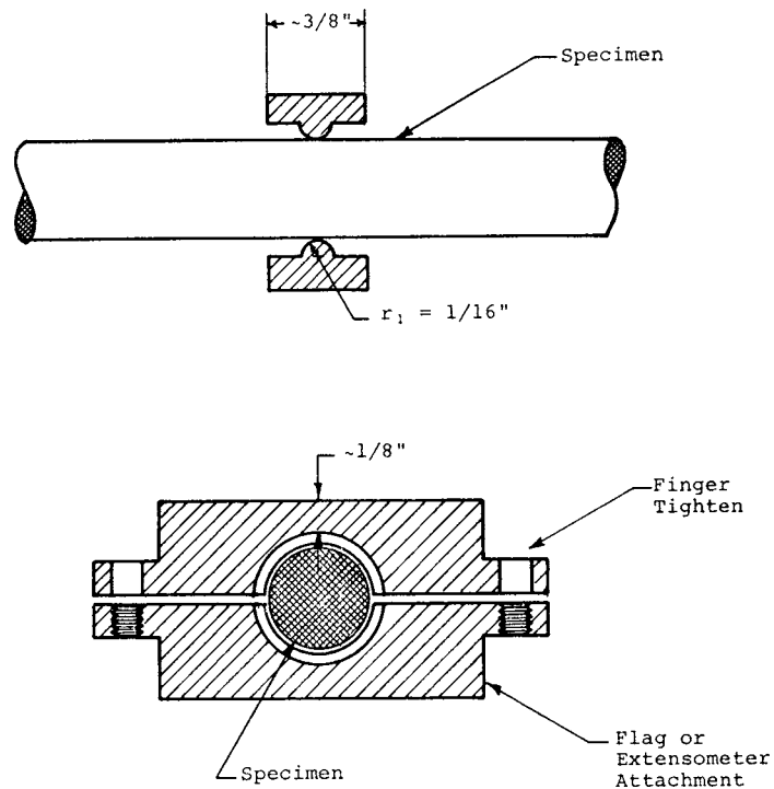
NOTE 1—Jig align to ensure precision gauge length; mount post or groove to match type of extensometer. FIG. 10 Attachment for Strain Flags or Extensometers to Provide Minimum Damage to Surface of Specimen
