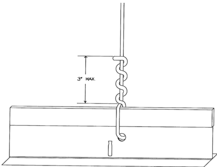
FIG. 6 Hanger Wire Tie Detail
