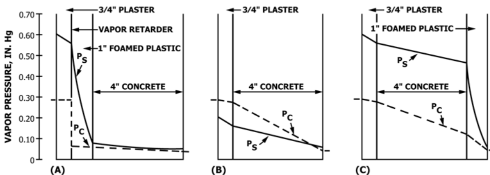
FIG. X1.2 Vapor Pressure Gradients of Modified Building Wall (5)
