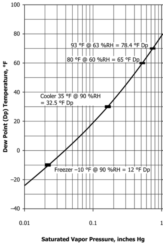
FIG. 1 Dew Point (Dp) Relation to Water Vapor Pressure
