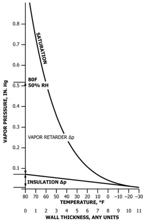
FIG. X1.3 Limiting Vapor Pressure Gradient Plot (3)
