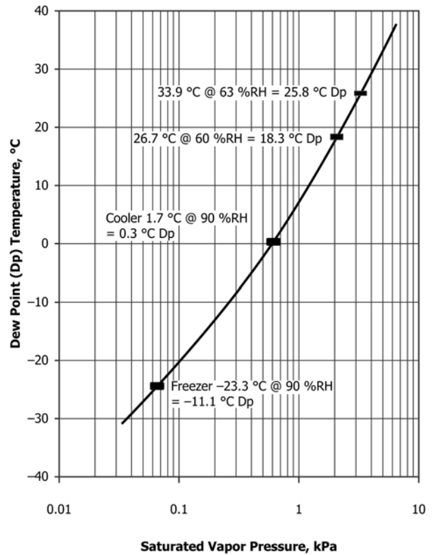
FIG. 1 Dew Point (Dp) Relation to Water Vapor Pressure
