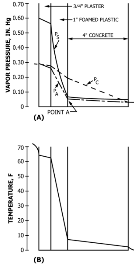
FIG. X1.1 Vapor Pressure and Temperature Gradients of Building Wall (5)
