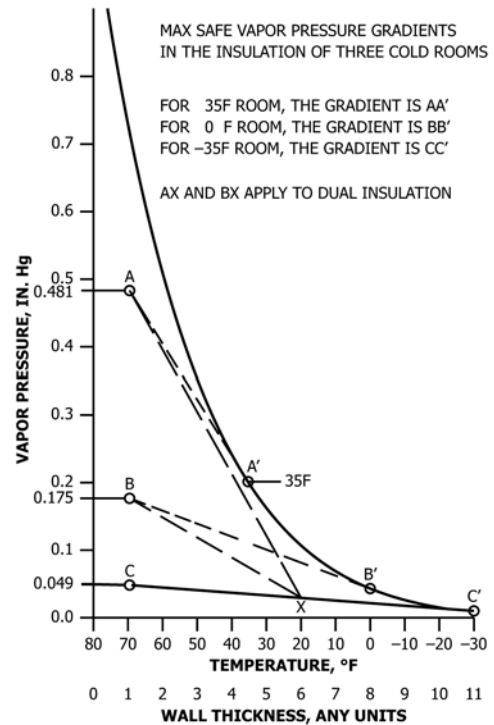
FIG. X1.4 Saturation Vapor Pressure vs. Temperature (3)
