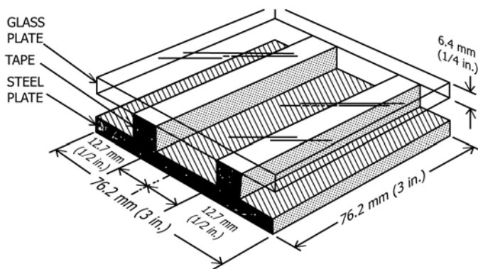
FIG. 1 Test Specimens Assembly
