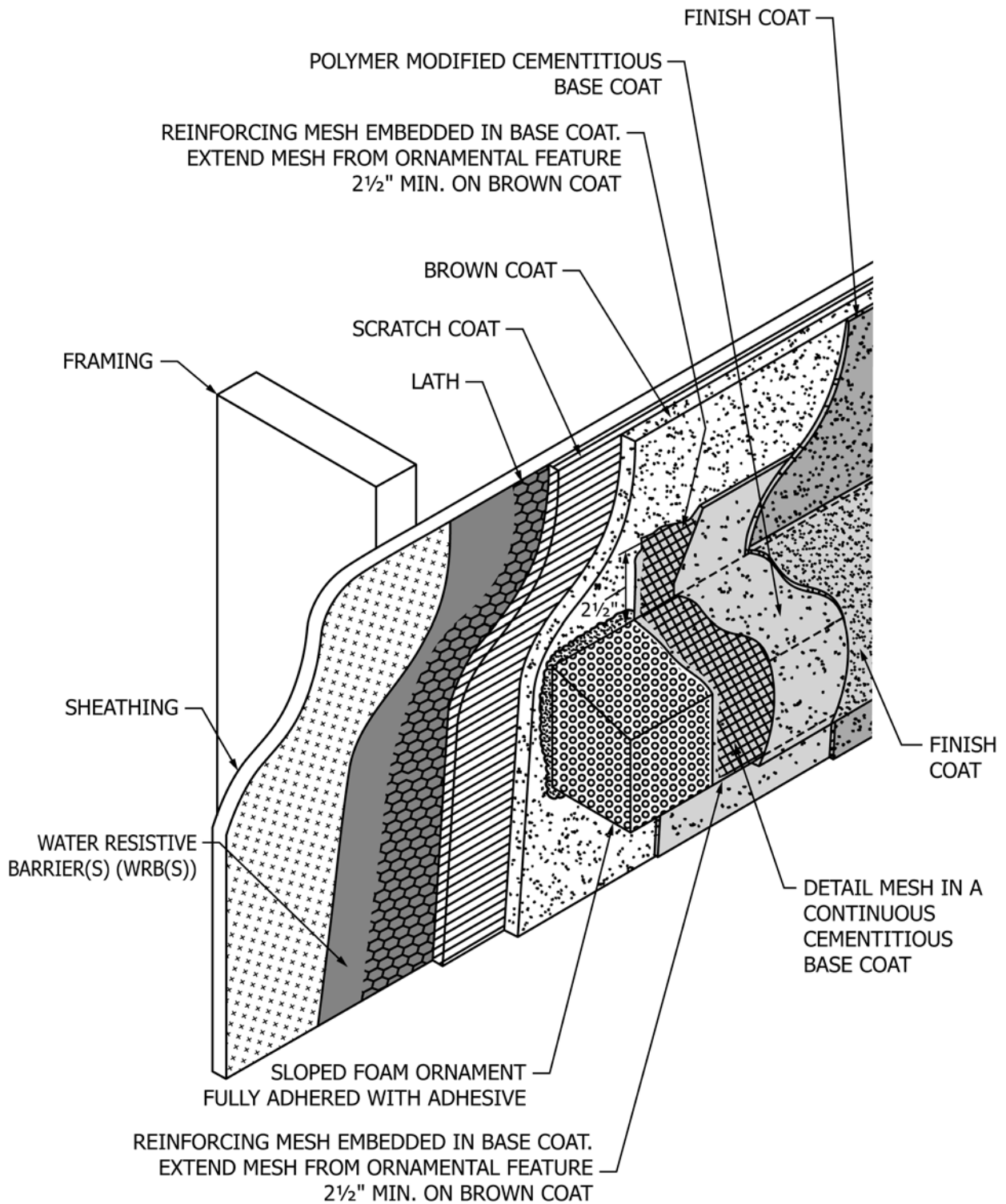
FIG. A2.1 Sample Detail of Ornamental Feature Consisting of Foam Plastic Core Encapsulated with Polymer Modified Cementitious Base Coat and Finish Coat
