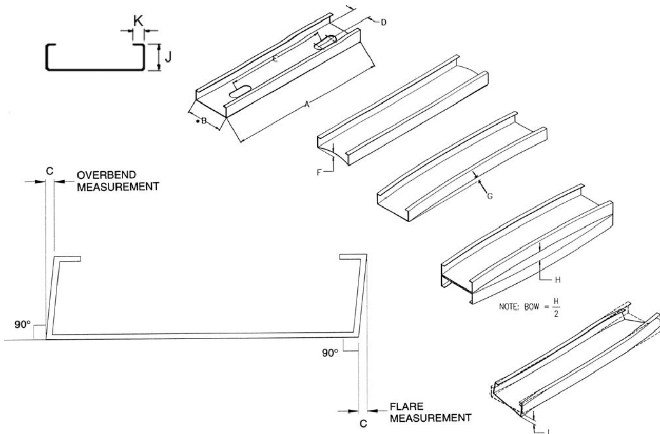
FIG. 1 Manufacturing Tolerances
