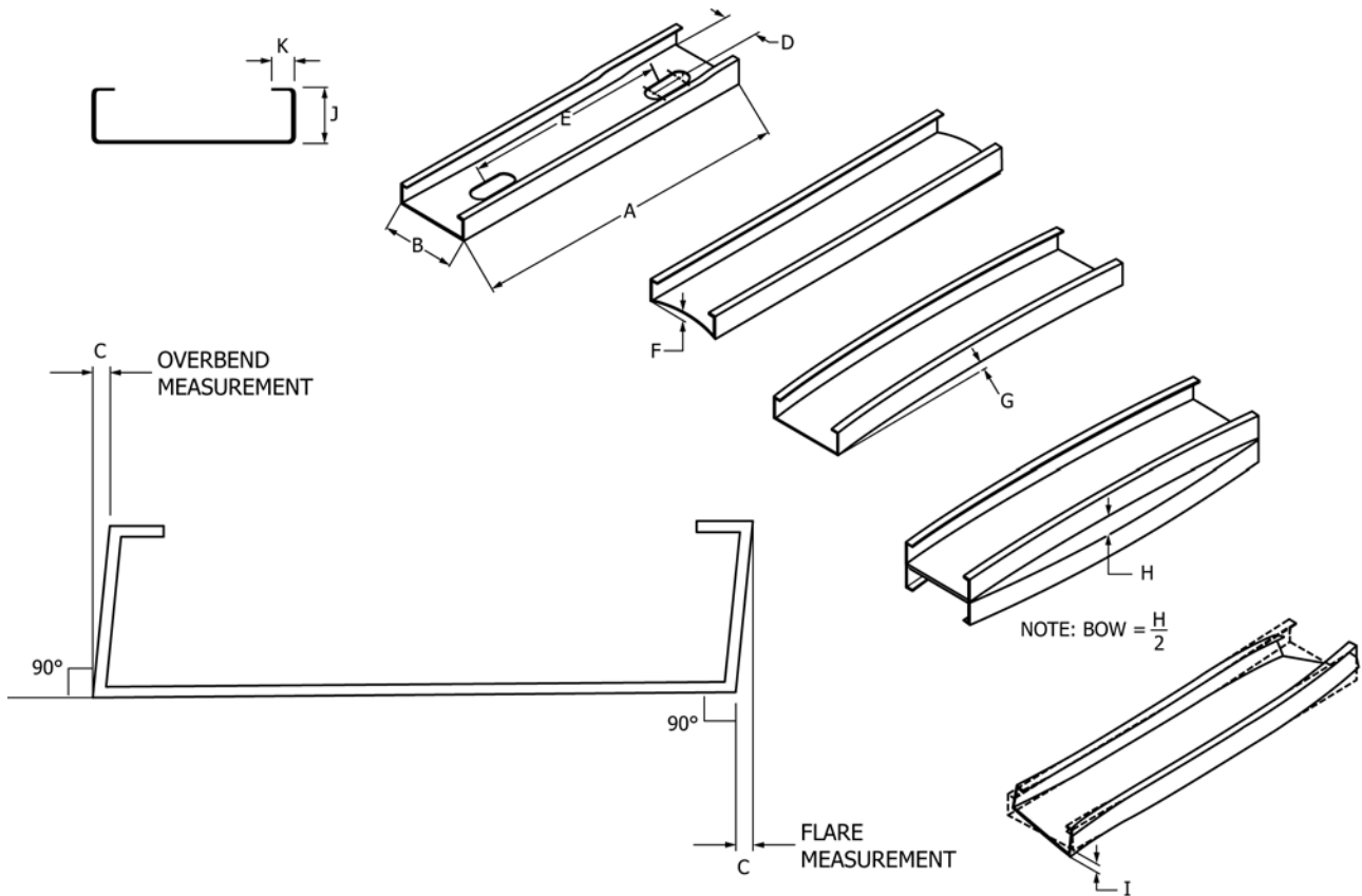
FIG. 1 Manufacturing Tolerances
