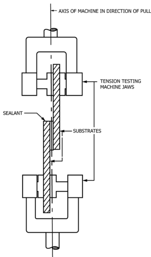
FIG. 4 Test Assembly Installed in Testing Machine
