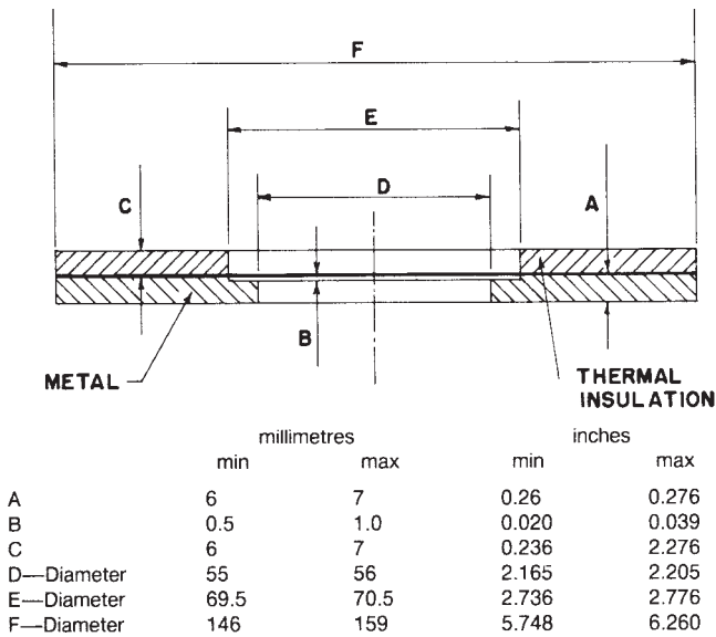
FIG. 2 Heating Plate
