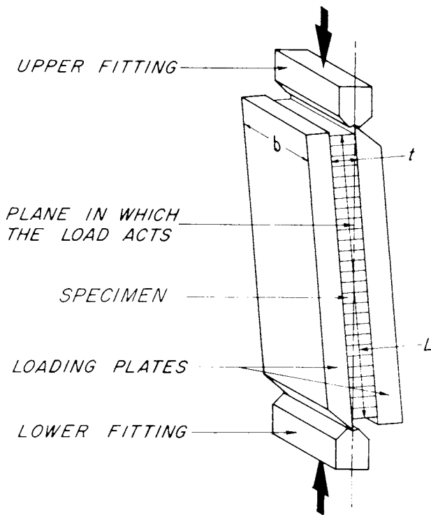
FIG. 26 Detail of Specimen and Loading Apparatus for Determining Interlaminar Shearing Properties
