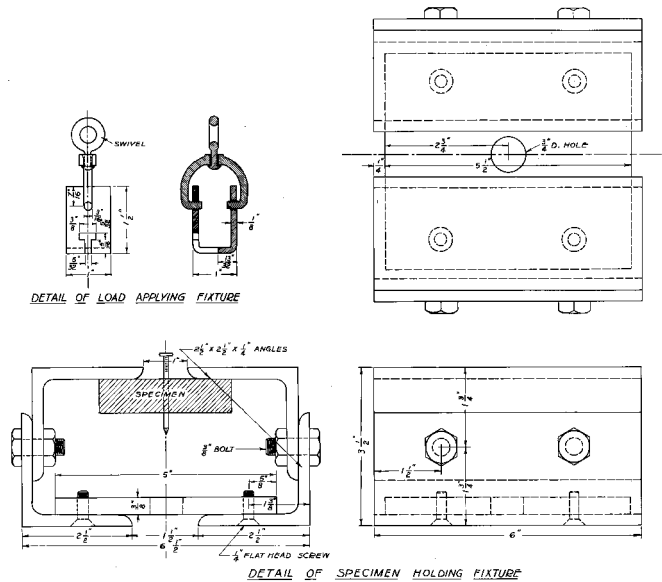
NOTE—1 in. = 25.4 mm. FIG. 14 Details of Testing Equipment for Measuring the Resistance of Nails to Direct Withdrawal
