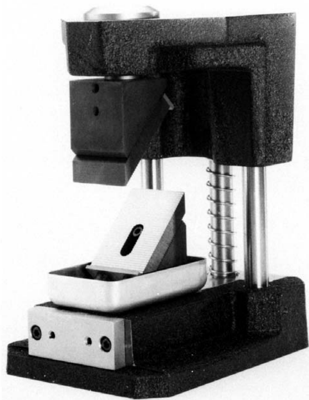
FIG. 32 Compression-Shear Device
