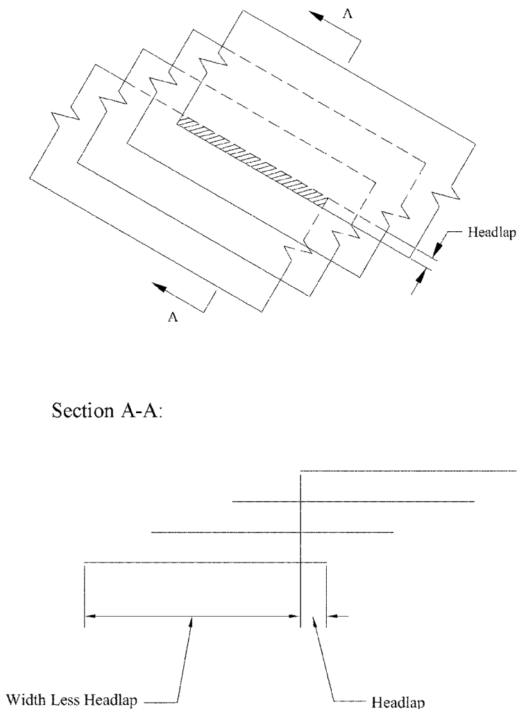
FIG. 1 Headlap in Multiple Sheet Roofing
