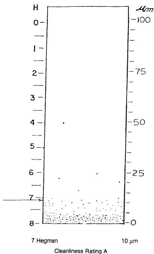
FIG. 4 i Typical Fineness Gage Pattern (continued)
