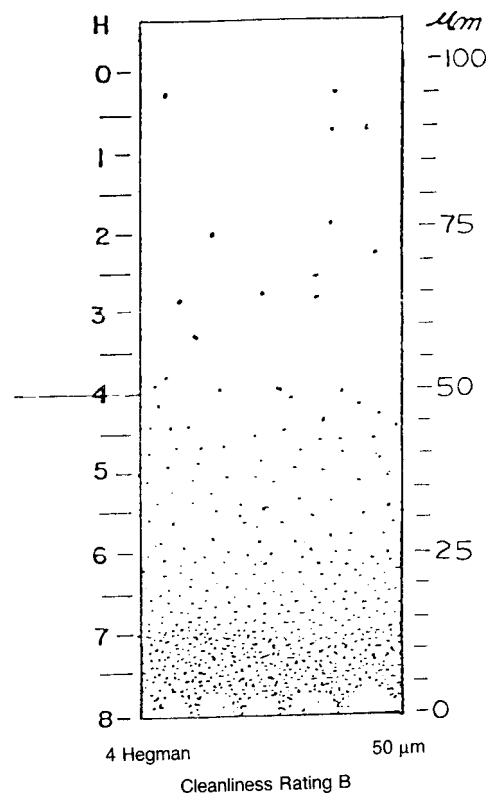
FIG. 4 d Typical Fineness Gage Pattern (continued)
