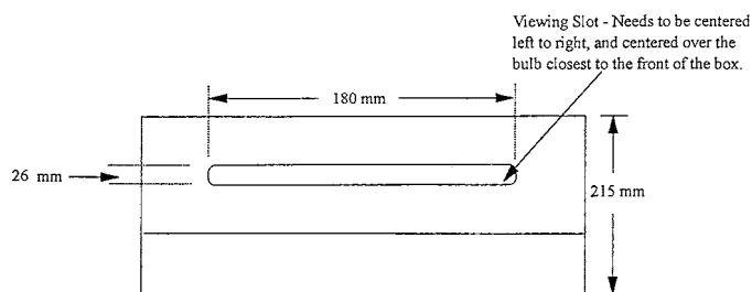
FIG. X1.1 Top View with Lid Removed
