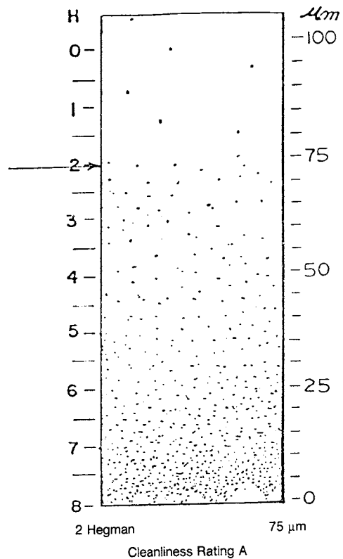
FIG. 4 b Typical Fineness Gage Pattern (continued)
