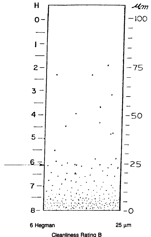
FIG. 4 g Typical Fineness Gage Pattern (continued)
