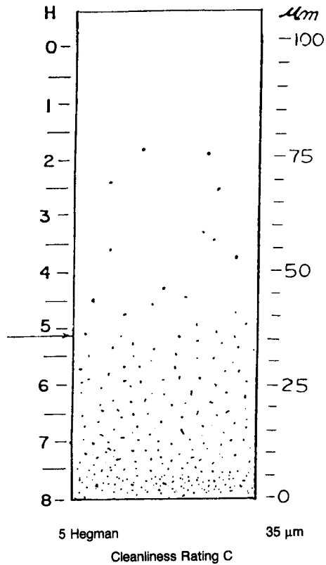
FIG. 4 e Typical Fineness Gage Pattern (continued)
