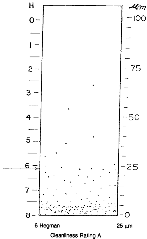
FIG. 4 f Typical Fineness Gage Pattern (continued)
