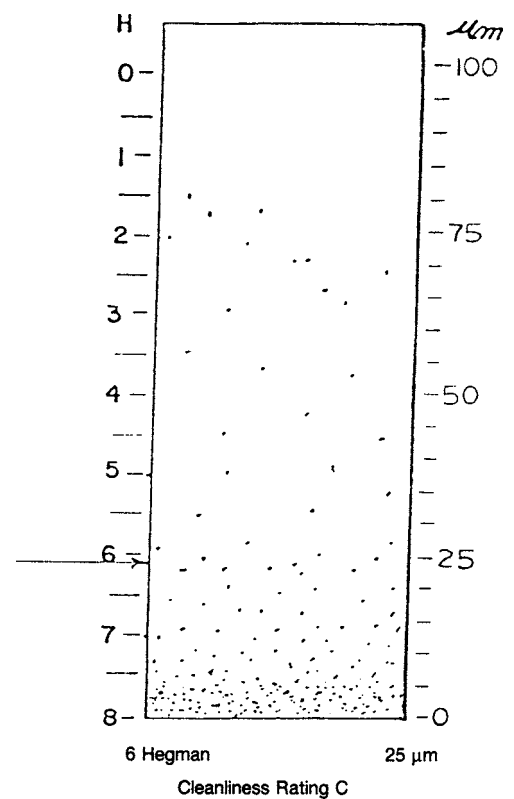
FIG. 4 h Typical Fineness Gage Pattern (continued)
