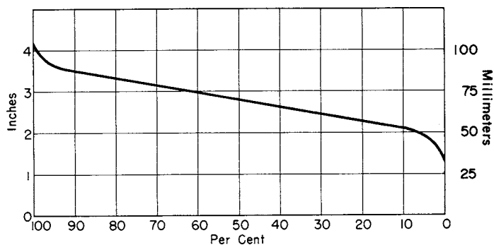
FIG. 2 Cumulative Staple Length Frequency Curve
