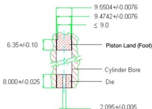
Figure # 2 - Dimensions of the cylinder bore, piston foot & standard die
