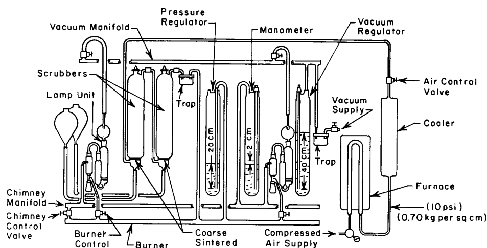
FIG. A2.1 Schematic Diagram of Purified Air Supply Manifold and Lamp System
