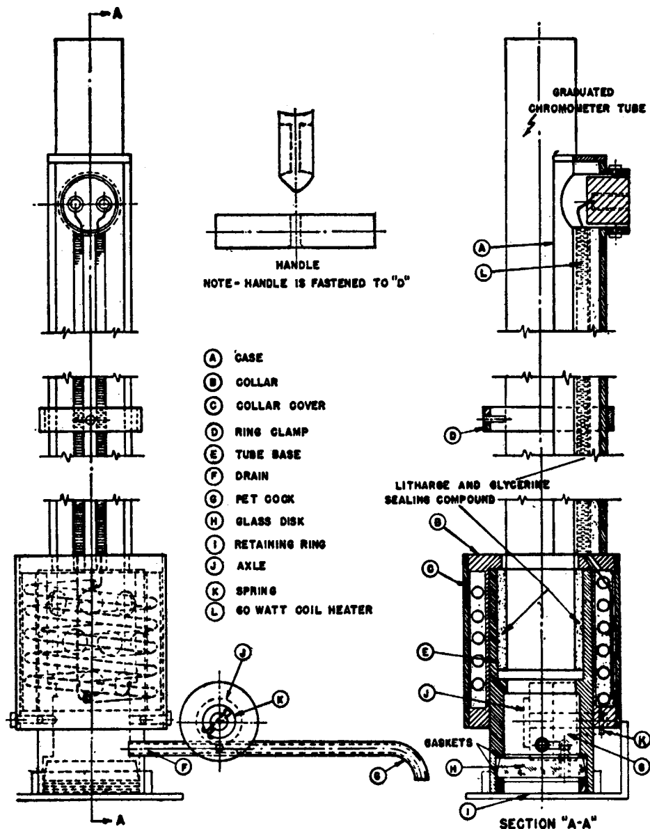
FIG. A1.2 Saybolt Chromometer Tube Heater
