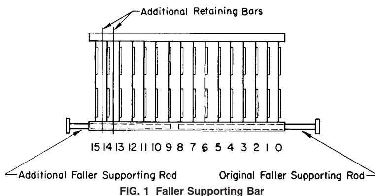
FIG. 1 Faller Supporting Bar
