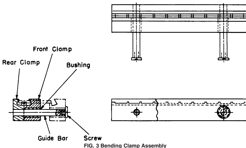
FIG. 3 Bending Clamp Assembly
