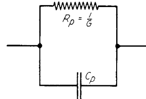
FIG. 3 Parallel Circuit
