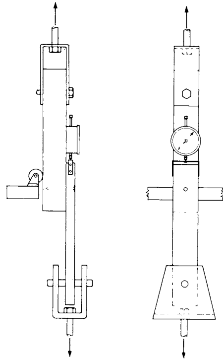
FIG. 3 Diagram of Assembly for Lateral Resistance Test of Nails, Staples, or Screws
