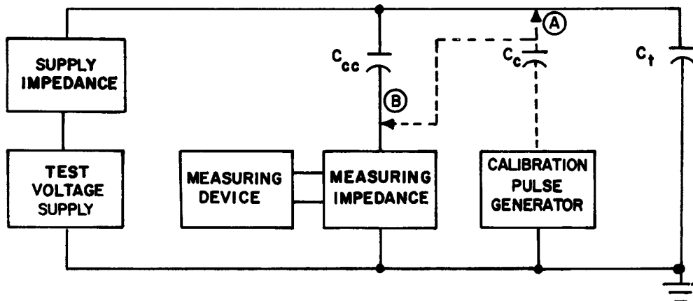
FIG. 1 Circuit No. 1
