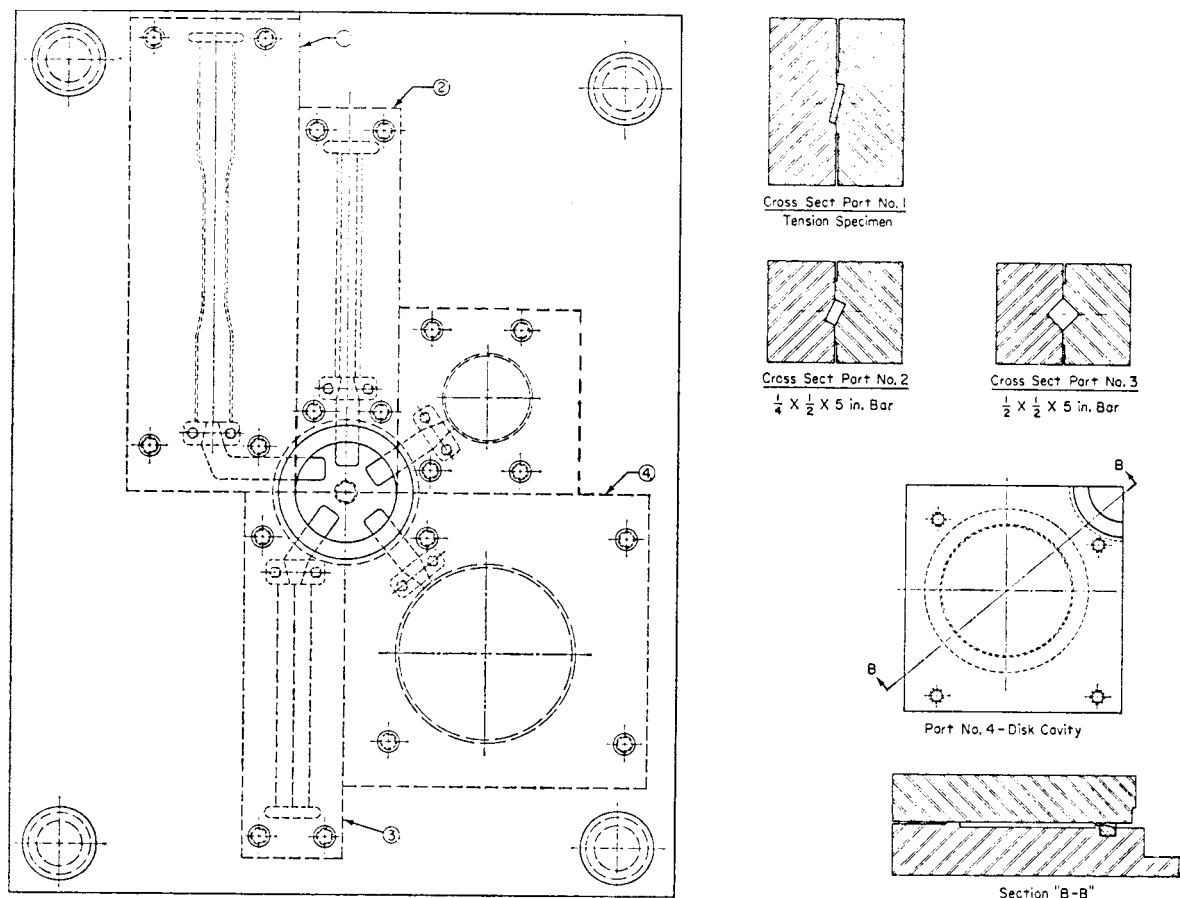
FIG. 1 Five-Cavity Transfer Mold for Thermosetting Plastic Test Specimens (Steam Cores Not Shown)
