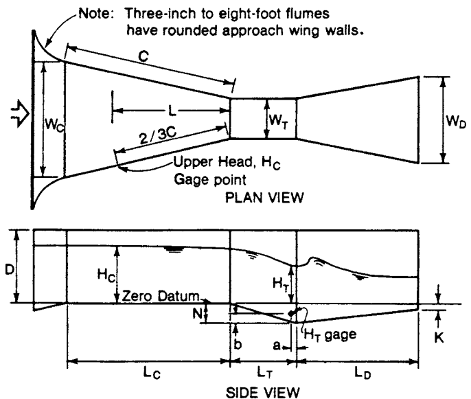
FIG. 1 Parshall Flume
