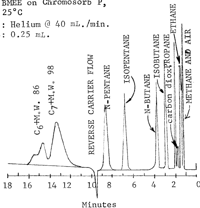
FIG. 4 Chromatogram of Natural Gas (BMEC Column) (See Annex A2)
