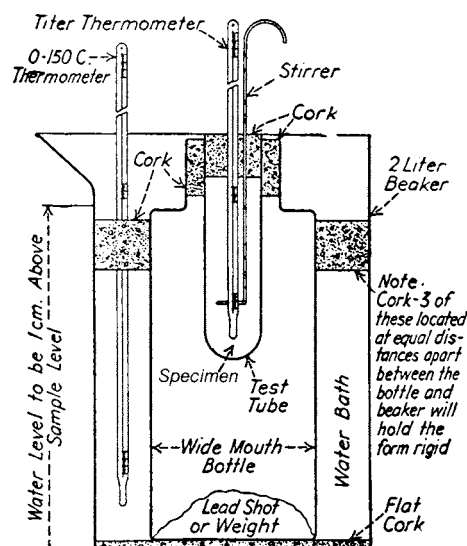
FIG. 1 Apparatus Assembly for Titer Test
