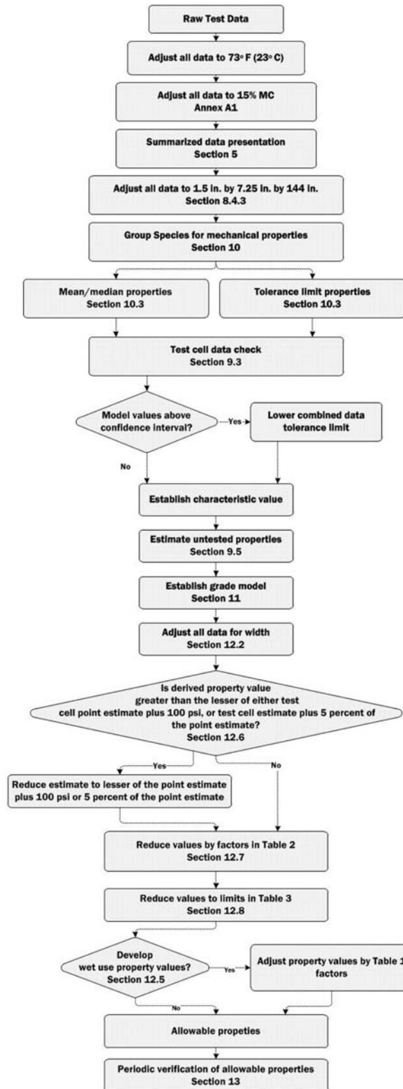
FIG. X3.1 Flow Diagram of Practice
