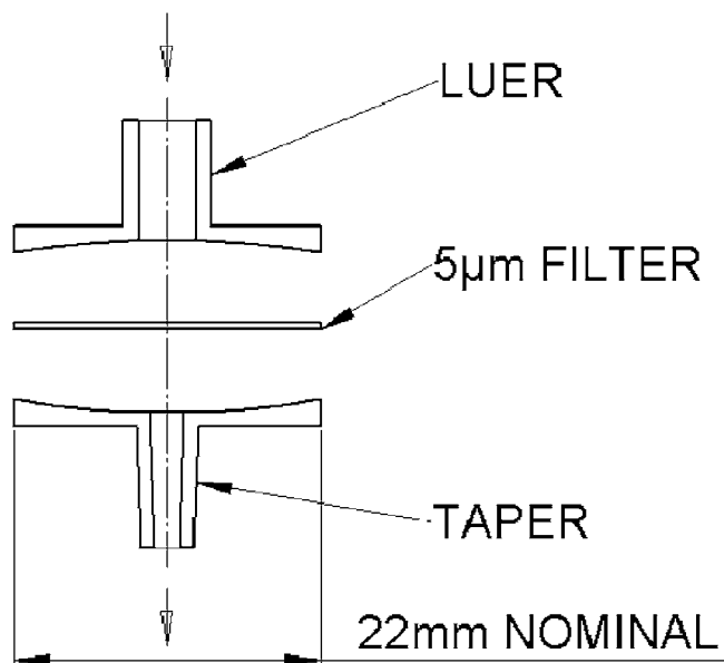
FIG. 3 Filter C
