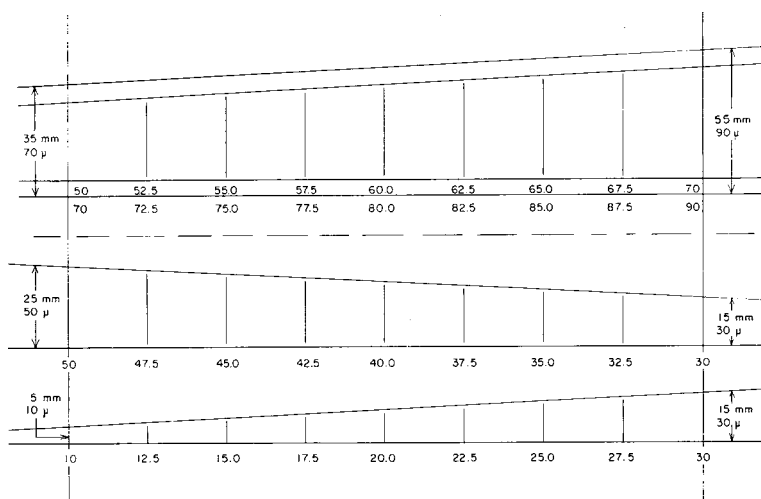
FIG. 3 Wedge Scale
