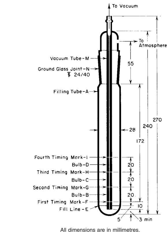
FIG. 4 Modified Koppers Vacuum Capillary Viscometer
