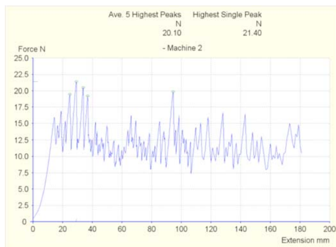
FIG. 3 Typical Tongue Tearing Force-Extension Curves for Individual Specimens (Typical woven cotton fabric)
