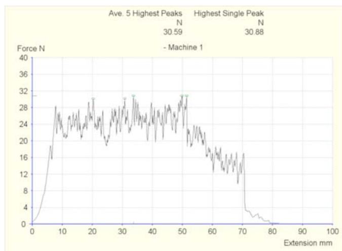
FIG. 5 Typical Tongue Tearing Force-Extension Curves for Individual Specimens (Typical non-woven fabric)
