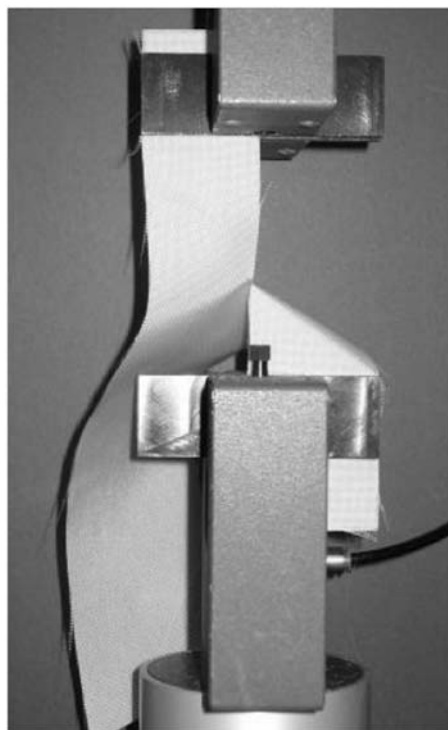
FIG. 2 Loading the Specimen in the Jaws (The slit is centered and vertically orientated. Each “leg” is secured in the jaw as shown. The two legs present opposite faces of the fabric to the operator.)
