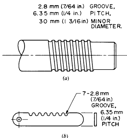
FIG. 7 Mandrel for Coil (a) and Coil Spacing Gauge (b)
