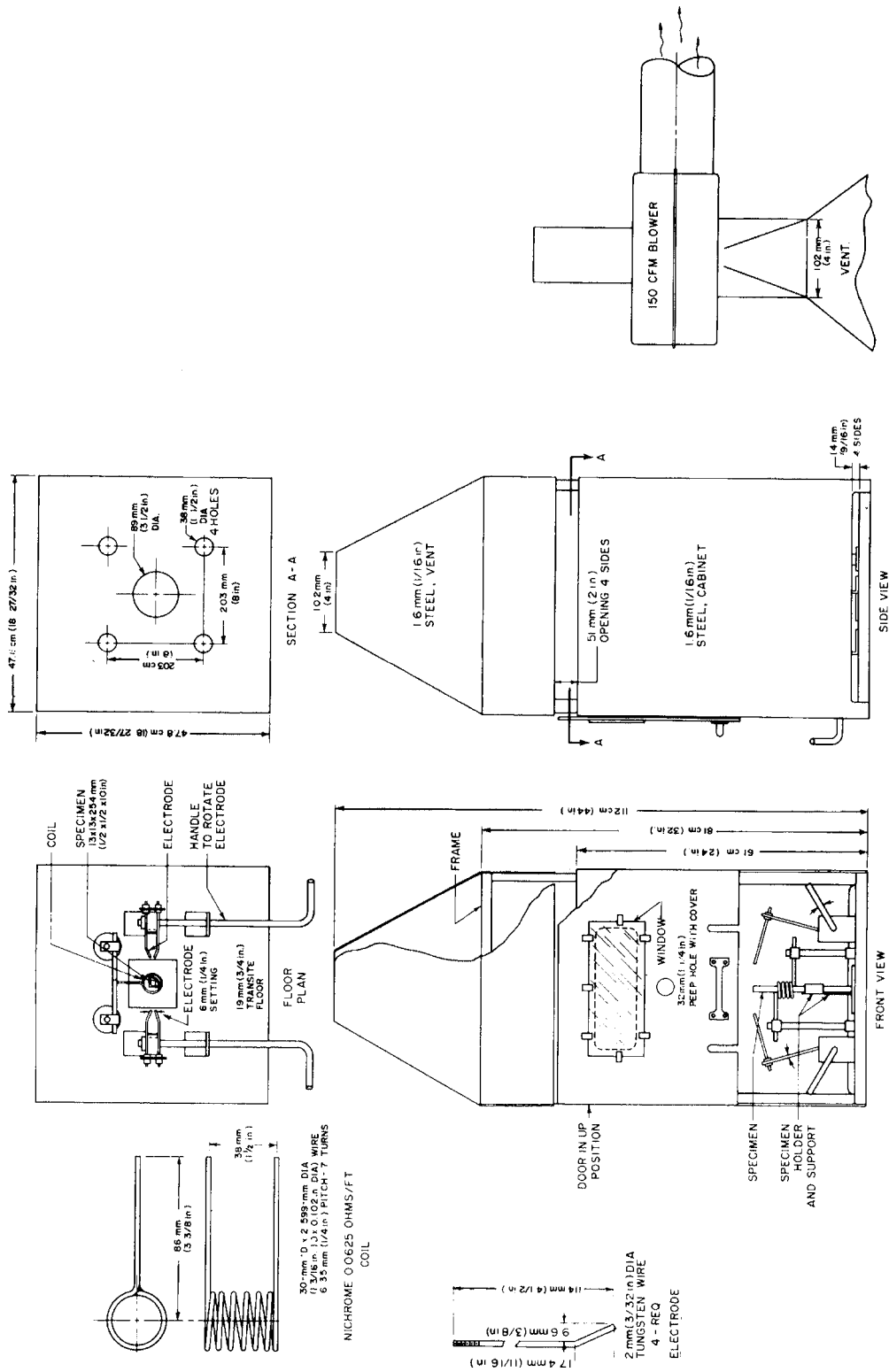
FIG. 5 Flame Cabinet
