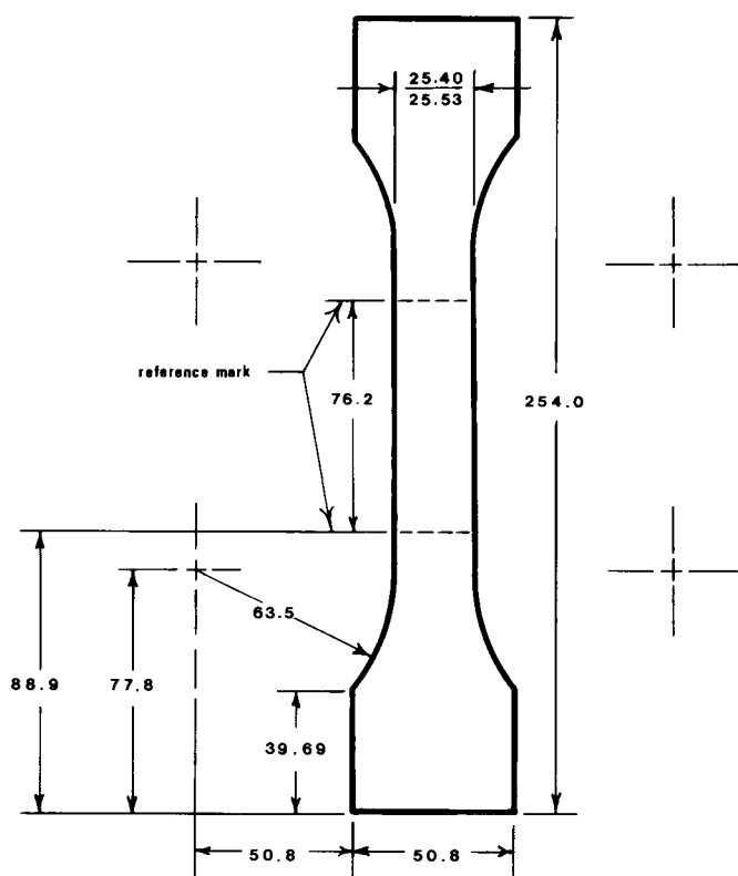
FIG. 1 Tension Test Specimen.
