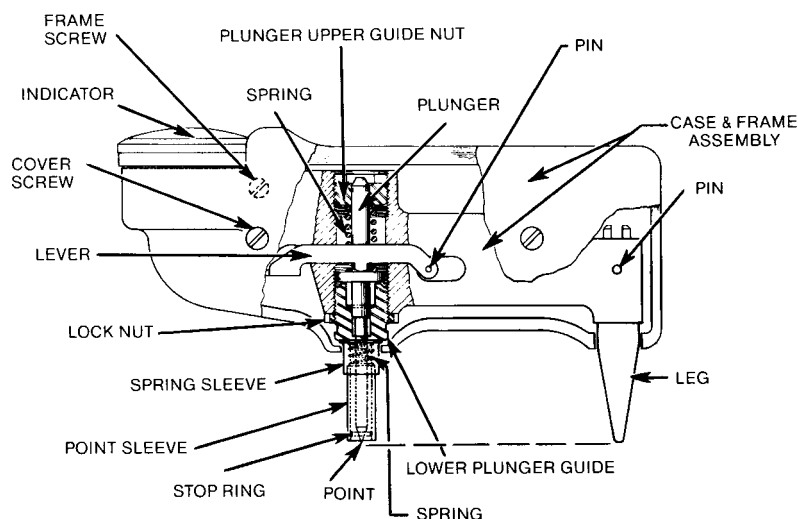
FIG. 2 Diagram of Barcol Impressor
