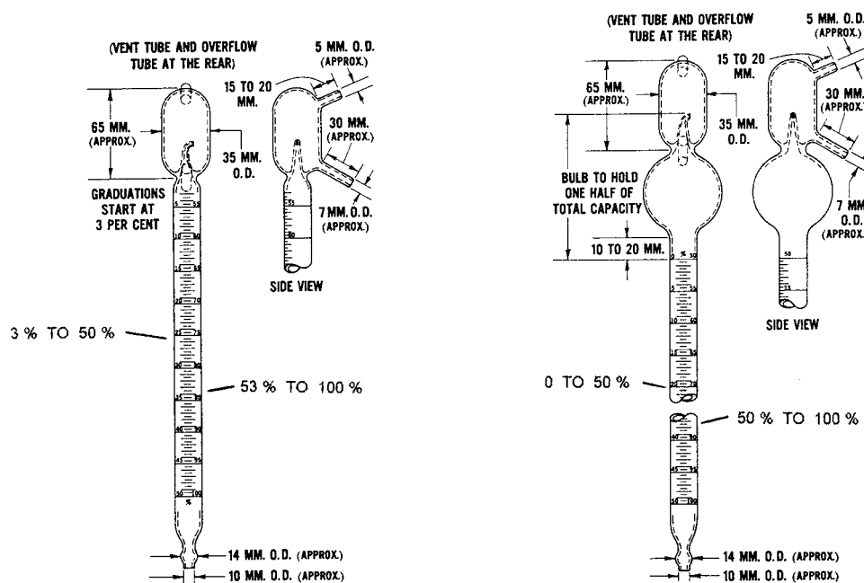
BURET WITHOUT BULB BURET WITH BULB FIG. X2.2 Typical Reference Material Dispensing Apparatus—Two Buret Style
