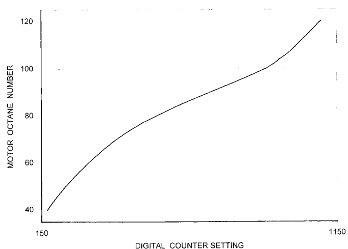
FIG. 3 Motor O.N. Versus Digital Counter Reading Characteristic
