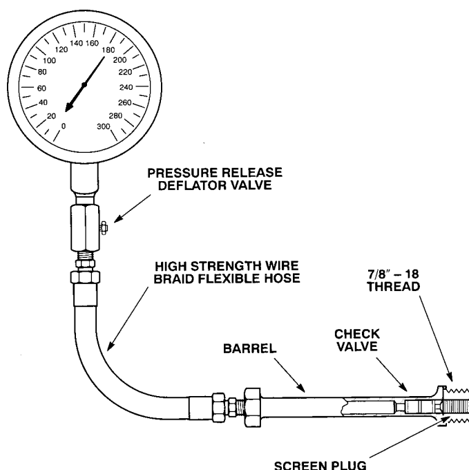
FIG. A2.4 Compression Pressure Gauge Assembly
