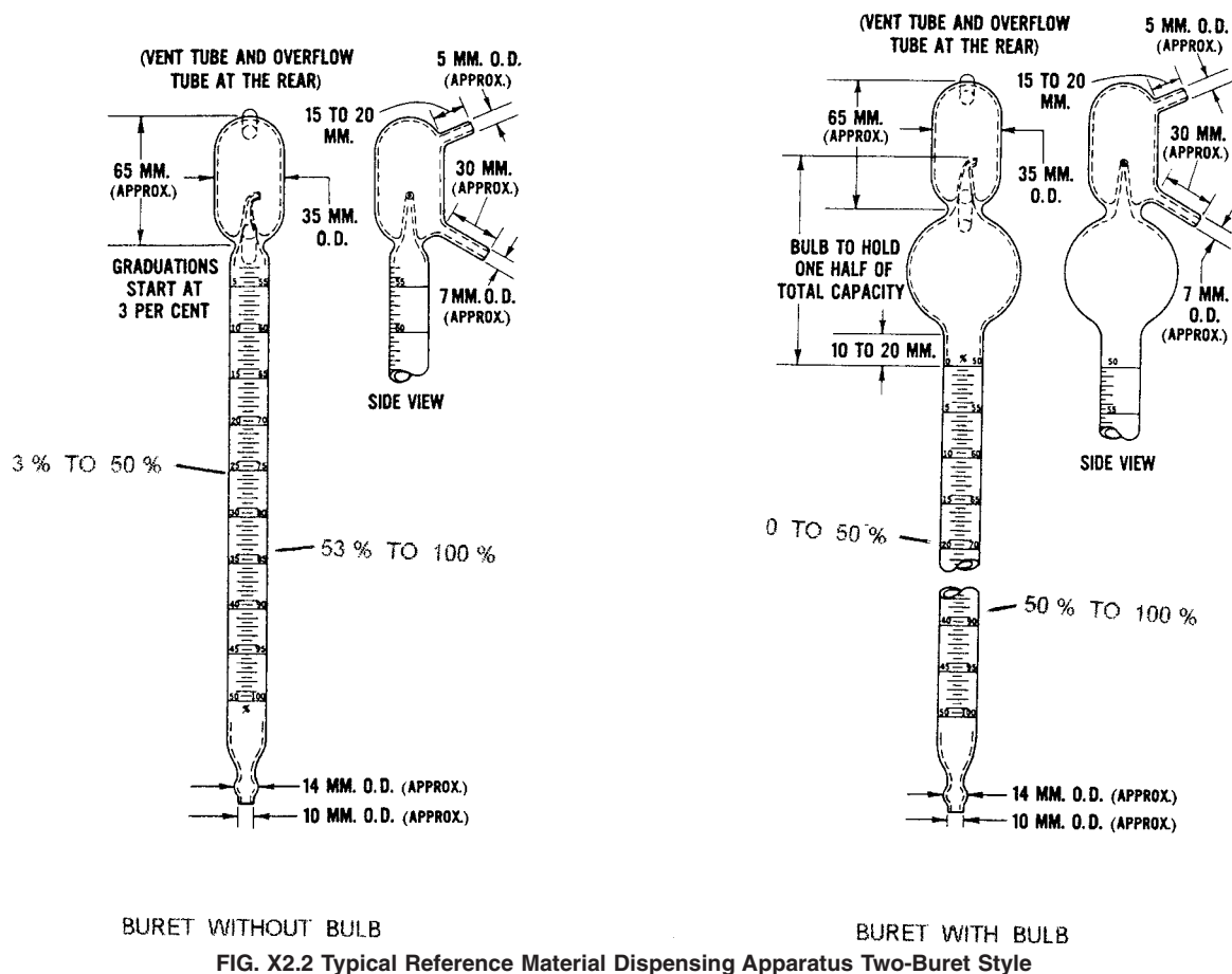
FIG. X2.2 Typical Reference Material Dispensing Apparatus Two-Buret Style
