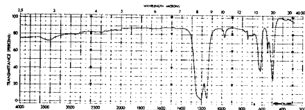
FIG. 9 Infrared Absorption Spectrum of a Typical Fluorocarbon Fiber
