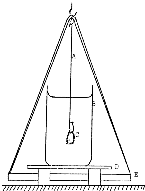
A) No. 34 Nichrome wire hook. D) Platform bridge. B) 250-ml beaker. E) Balance pan. C) Sample skein.
