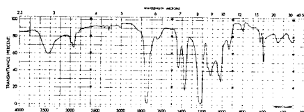
FIG. 14 Infrared Absorption Spectrum of a Typical Nitril Fiber
