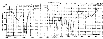
FIG. 21 Infrared Absorption Spectrum of a Typical Spandex Fiber
