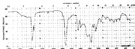
FIG. 5 Infrared Absorption Spectrum of a Typical Anidex Fiber
