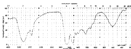
FIG. 23 Infrared Absorption Spectrum of a Typical Vinal Fiber
