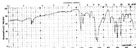
FIG. 19 Infrared Absorption Spectrum of a Typical Saran Fiber
