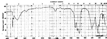
FIG. 7 Infrared Absorption Spectrum of a Typical Asbestos Fiber
