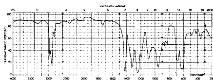
FIG. 24 Infrared Absorption Spectra of Typical Vinyon Fibers
