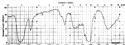
FIG. 8 Infrared Absorption Spectrum of a Typical Native Cellulosic Fiber
