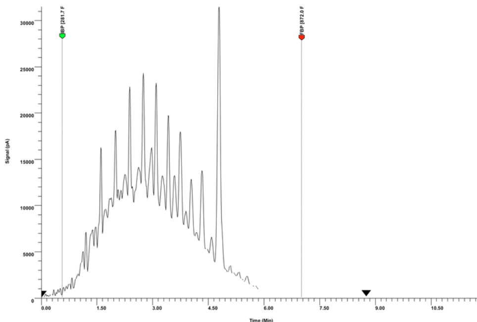
FIG. 9 Chromatogram of a Biodiesel (B-10) mixture
