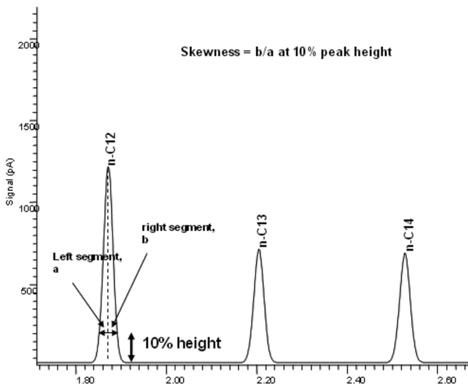
FIG. 4 Determination of Peak Skewness
