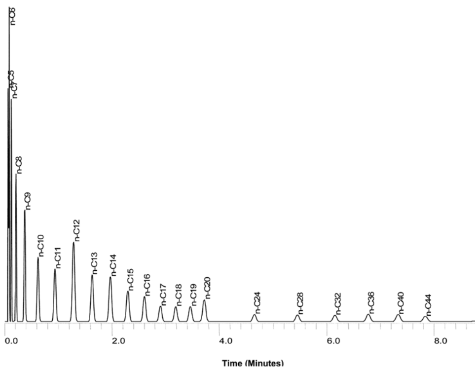
FIG. 5 Typical Retention Time Calibration (Columns 1-3, Table 8)
