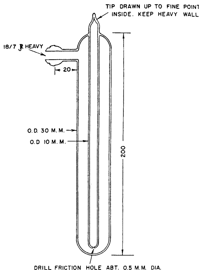
FIG. A6.3 Vacuum Manometer
