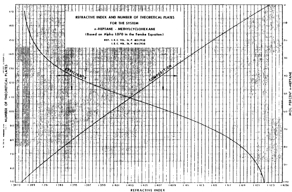
FIG. A1.3 Refractive Index
